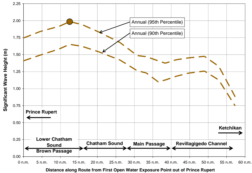
Figure 1: Significant wave heights along the Southern Gateway route
