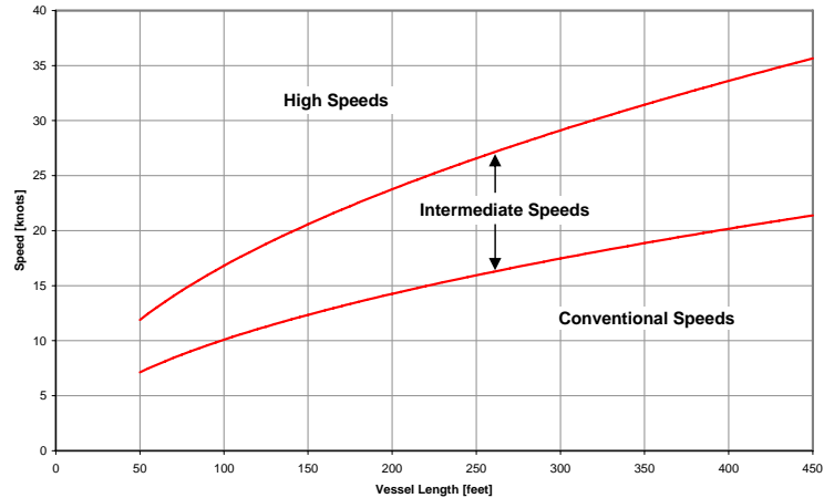
Figure 7: Ratio of speed to vessel length by vessel class
